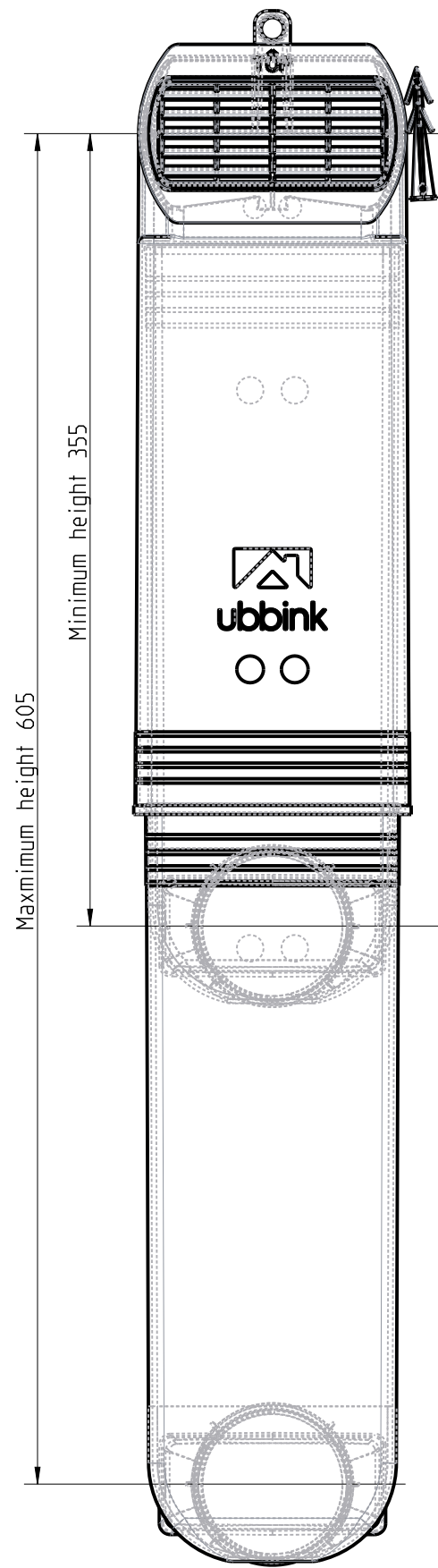
Adjustable height
