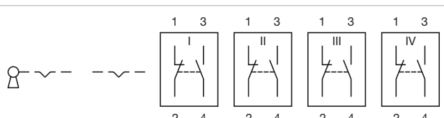
Wiring diagram 114
