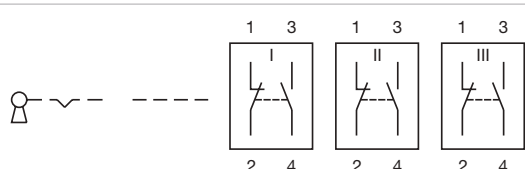
Wiring diagram 111
