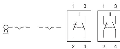
Wiring diagram 108
