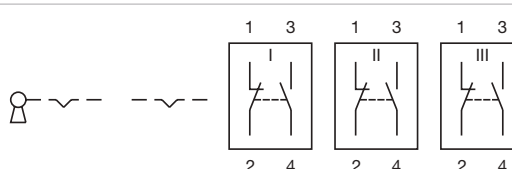
Wiring diagram 113
