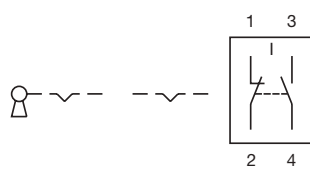
Wiring diagram 107
