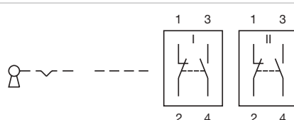
Wiring diagram 109
