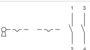
Wiring diagram 108
