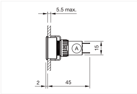
Dimensions [mm] A = Plug-in terminal 2.8 mm x 0.5 mm
