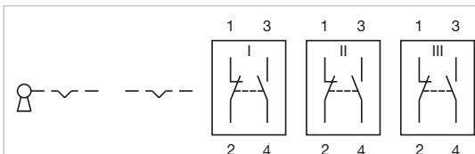
Wiring diagram 113
