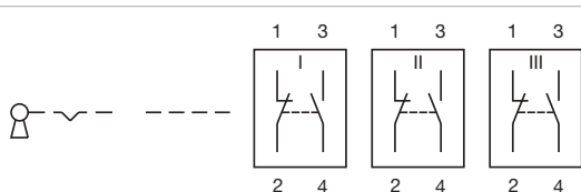
Wiring diagram 111
