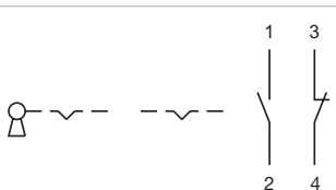
Wiring diagram 108
