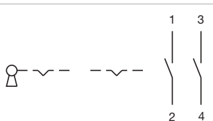
Wiring diagram 109
