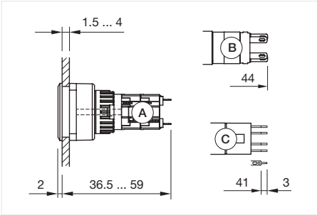
Dimensions [mm] A = Solder terminal B = Plug-in terminal 2.8 mm x 0.5 mm C = Universal terminal 2.0 mm x 0.5 mm
