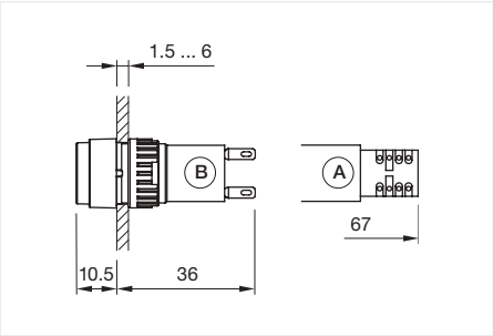
Dimensions [mm] A = Solder terminal B = Plug-in terminal 2.8 mm x 0.5 mm
