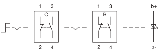
Wiring diagram 286
