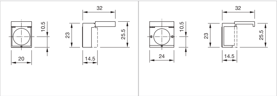
Dimensions [mm] For Part No. 51-920
