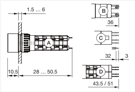
Dimensions [mm] A = Solder terminal B = Plug-in terminal 2.8 mm x 0.5 mm C = Universal terminal 2.0 mm x 0.5 mm D = Universal-Solder terminal
