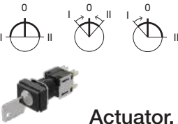
Actuator, Front dimension 24 mm x 18 mm
