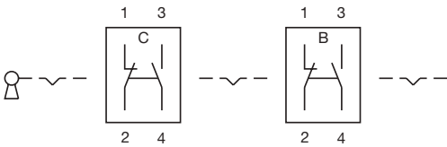
Wiring diagram 262
