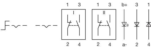
Wiring diagram 284
