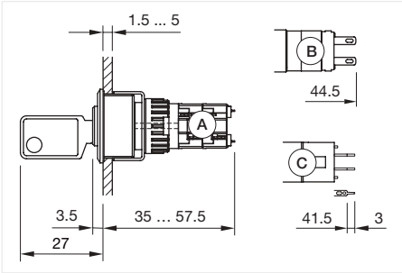
Dimensions [mm] A = Solder terminal B = Solder terminal 2.8 mm x 0.5 mm C = Universal terminal 2.0 mm x 0.5 mm
